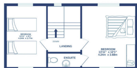
1ST FLOOR 398 sq.ft. (37.0 sq.m.) approx.
